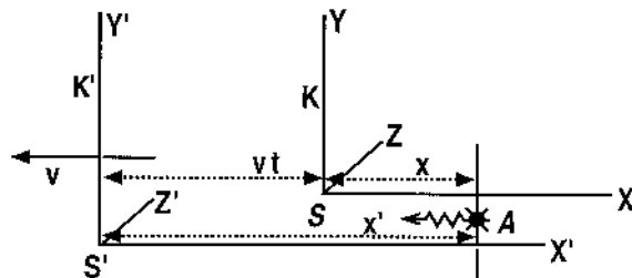
Fig.1.- Galilean systems: Observers in the stationary (K) and moving (K') frames are at the origins S and S' respectively
